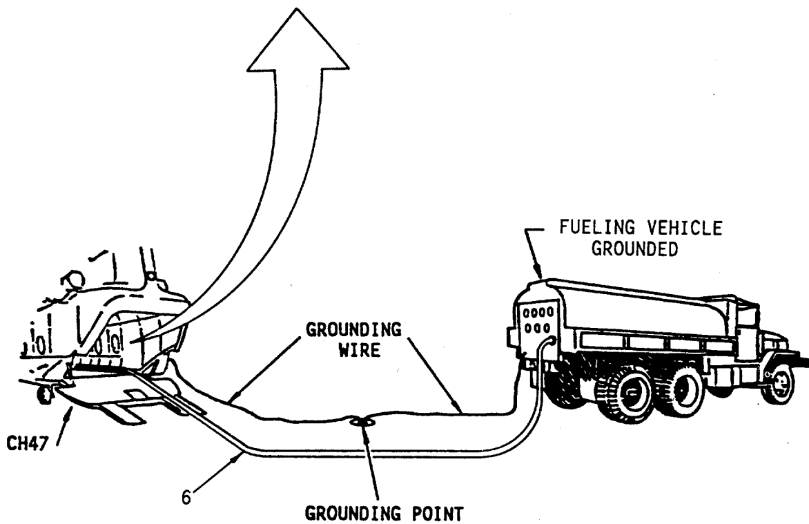
Figure 3-2. Pressure Refueling
