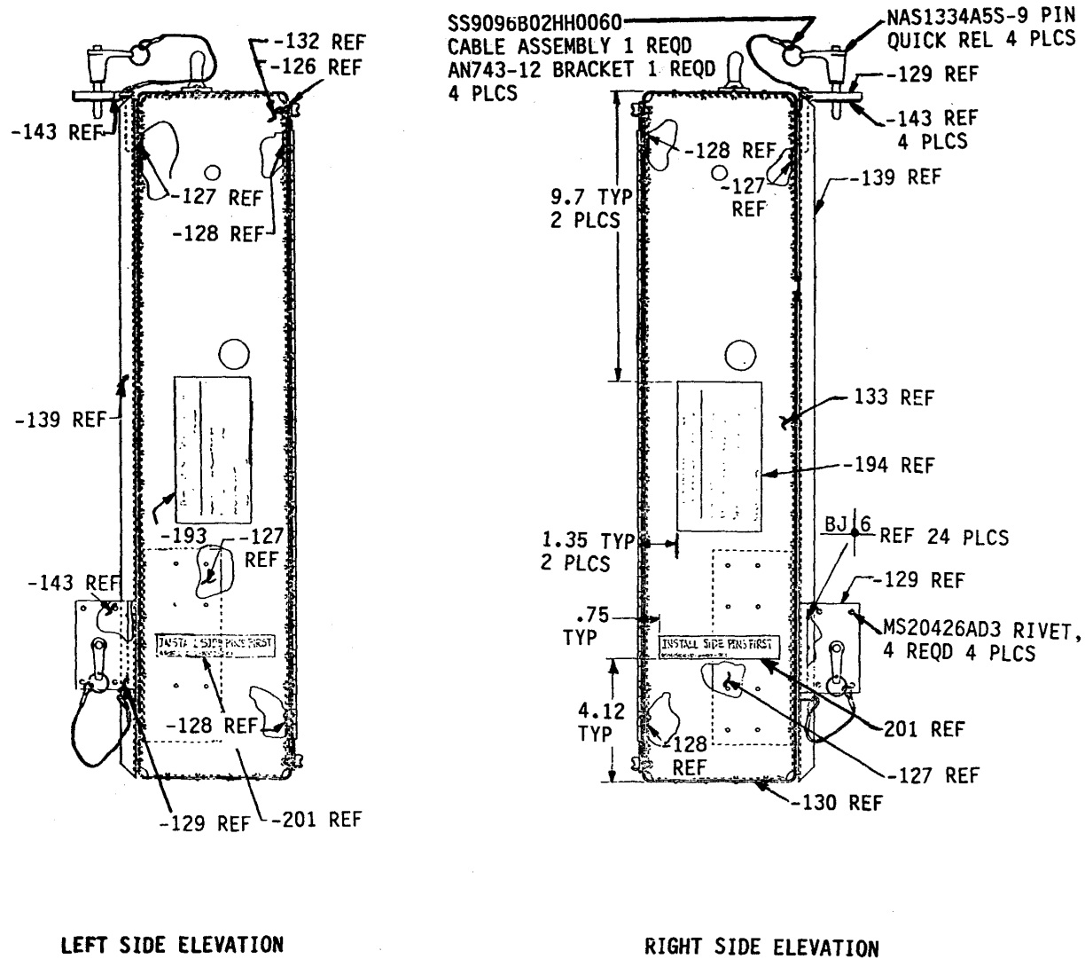
Figure E-8. Fabrication of Box Assembly, P/N 85SDSCC-D-0007-104 (Sheet 2 of 3)
